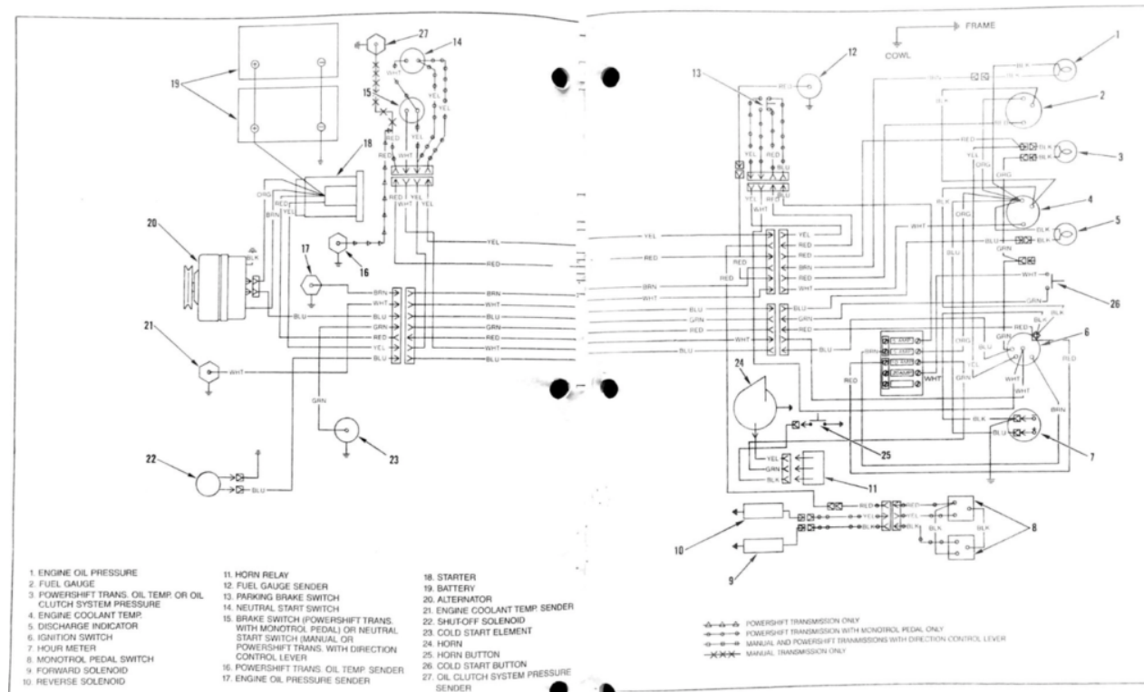
FIGURE 3. ELECTRICAL SCHEMATIC (DIESEL, PERKINS 4.2482)
